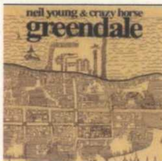
Greendale Website
